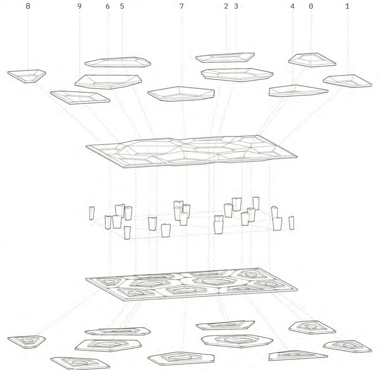
Structural columns defined at the nodal intersections of the tessellation
